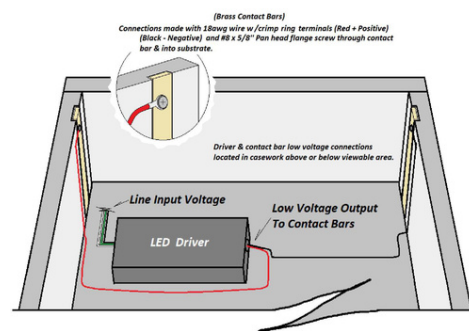
Adjustable Shelf Light "ASL" Driver, contact bar and wire lead set mounting illustration (Example)
